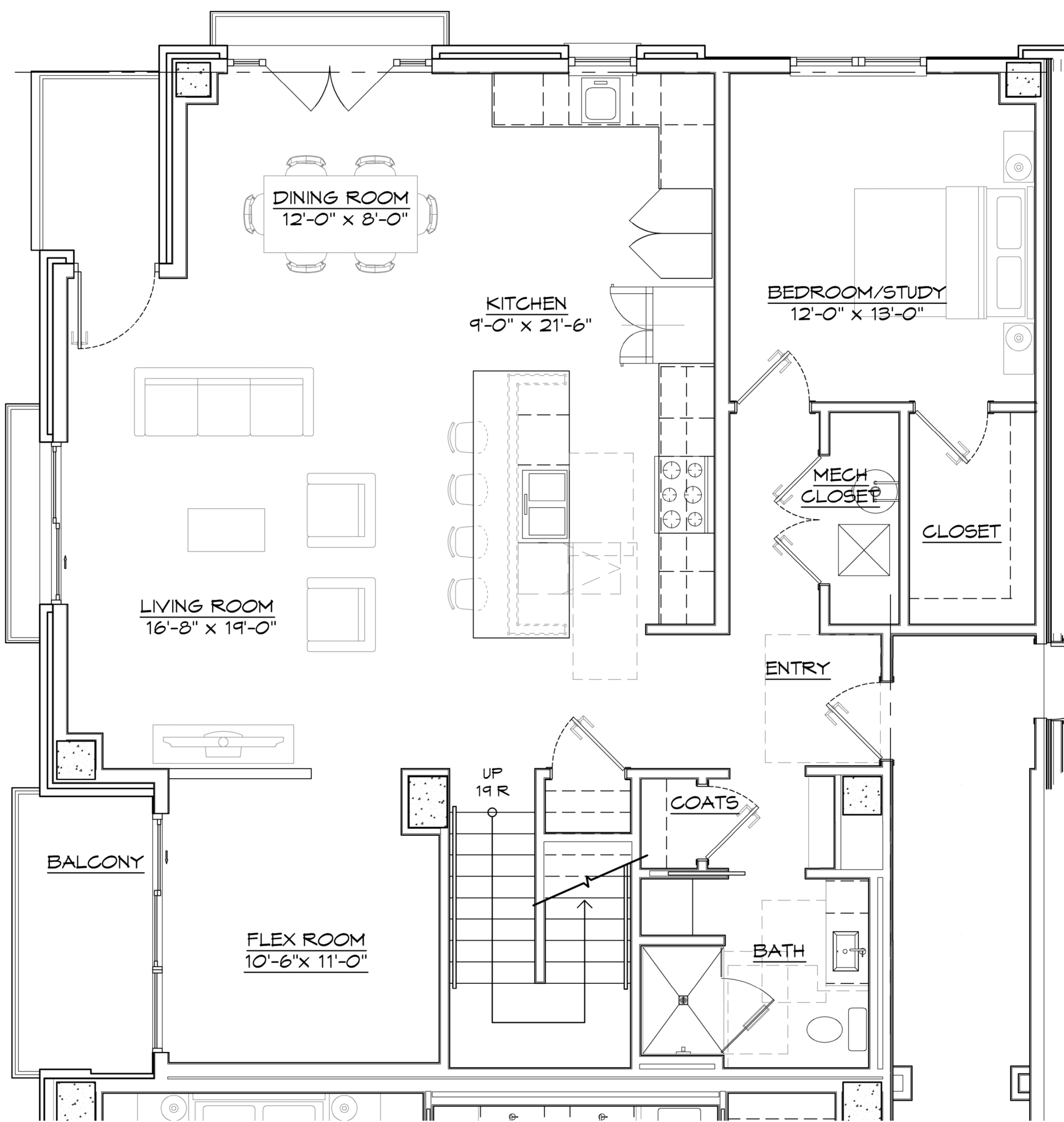
01 | CONDO UNIT 5 (Entry Level) 2649 NSF SCALE: 1/4" = 1'-0"
