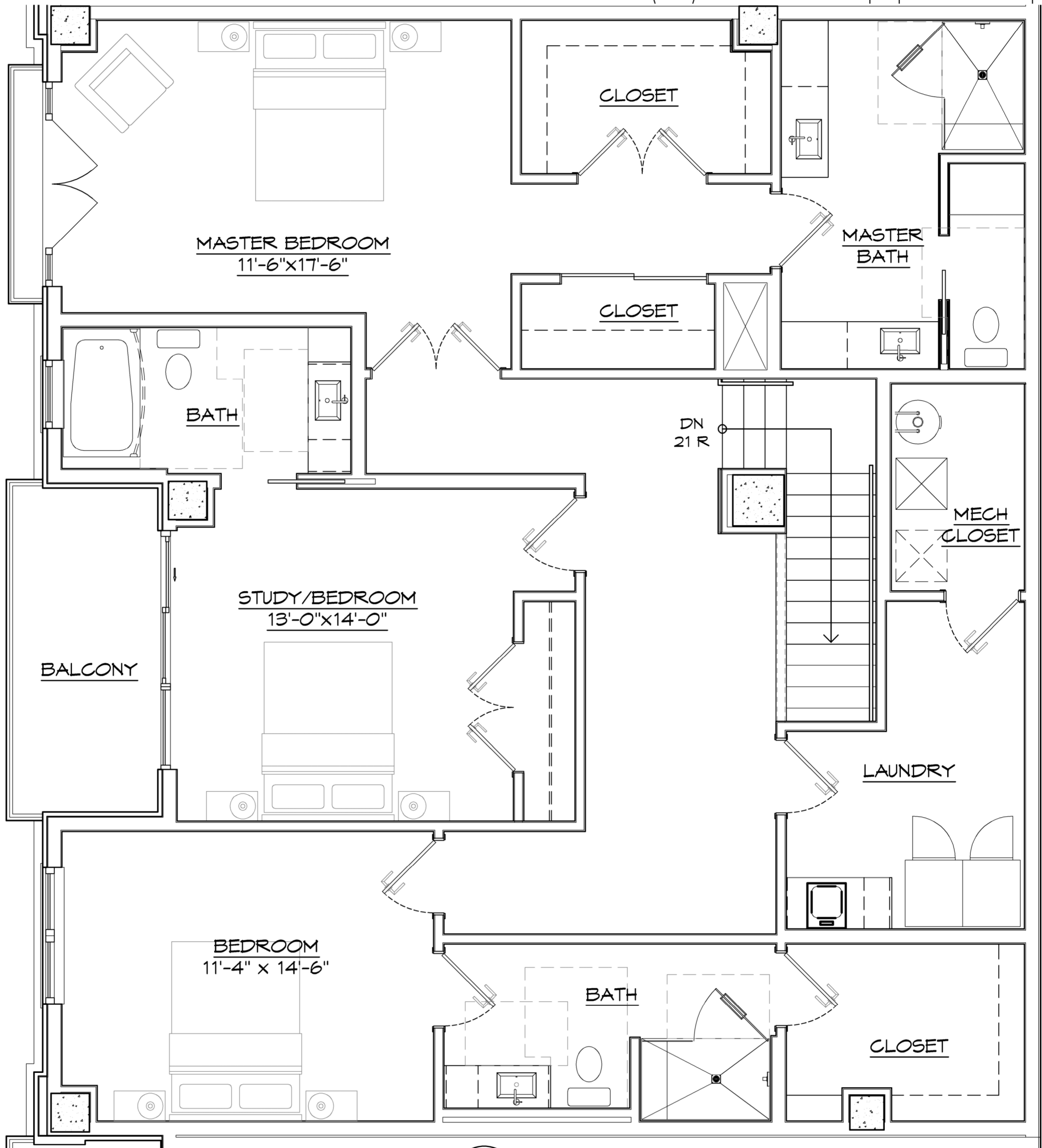
01 | CONDO UNIT 7 (Upper Floor) 2930 NSF SCALE: 1/4" = 1'-0" NORTH
